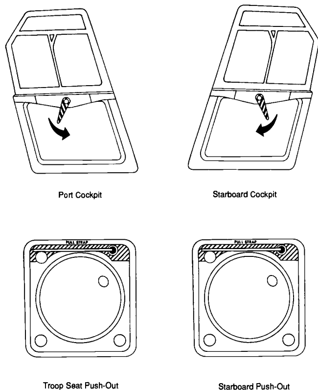
Fig. 3. Hatches and windows in the Labrador helicopter.
