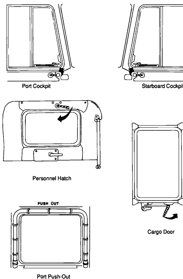
Fig. 2. Hatches and windows in the Sea King helicopter.
